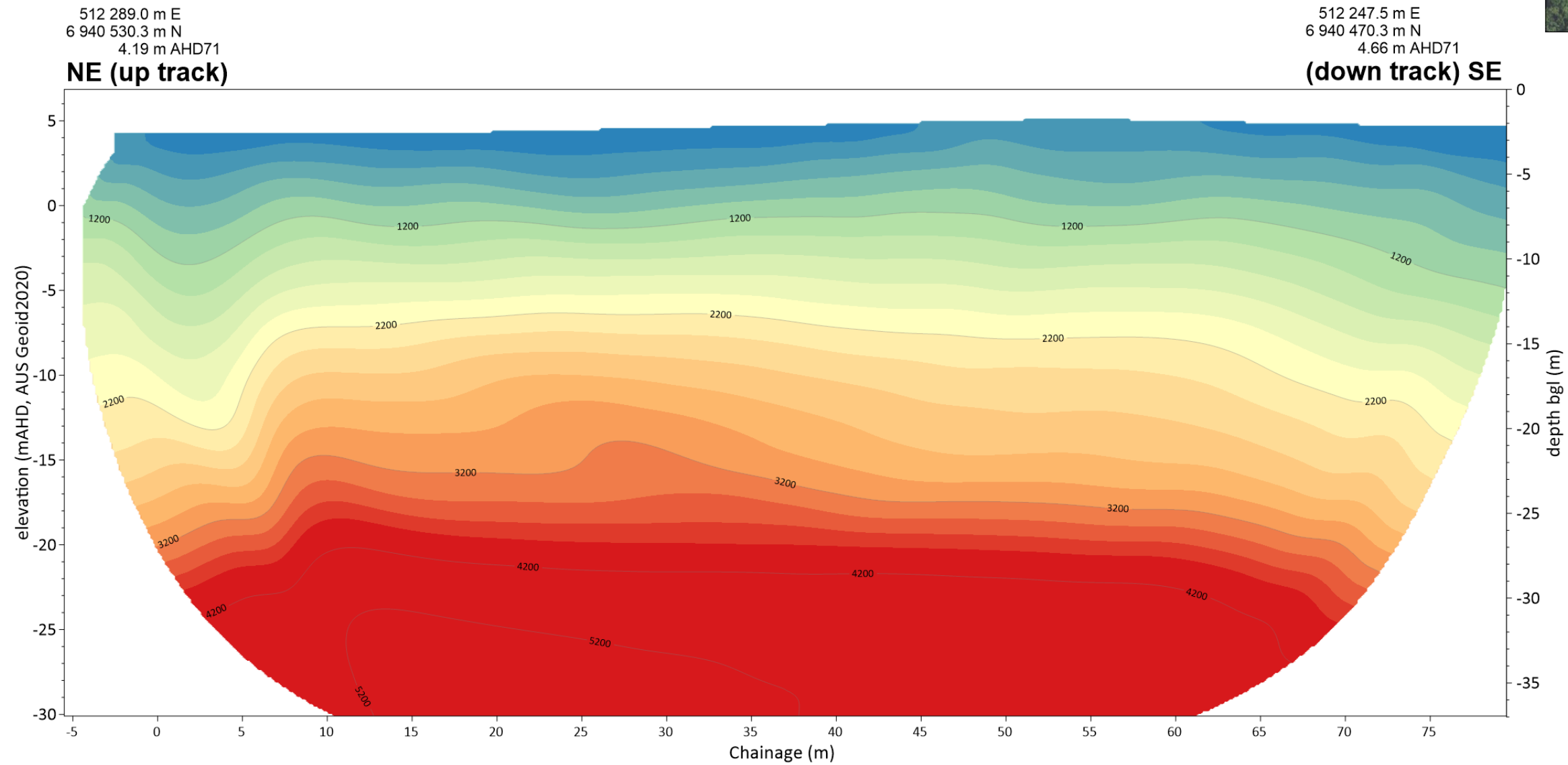
Seismic Line SR AU-GP 147
